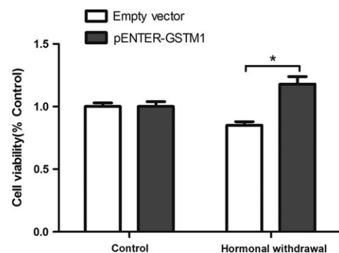
Figure 4 Effect of GSTM1 on endometrial epithelial cell (EEC) viability following hormone treatment and withdrawal.
