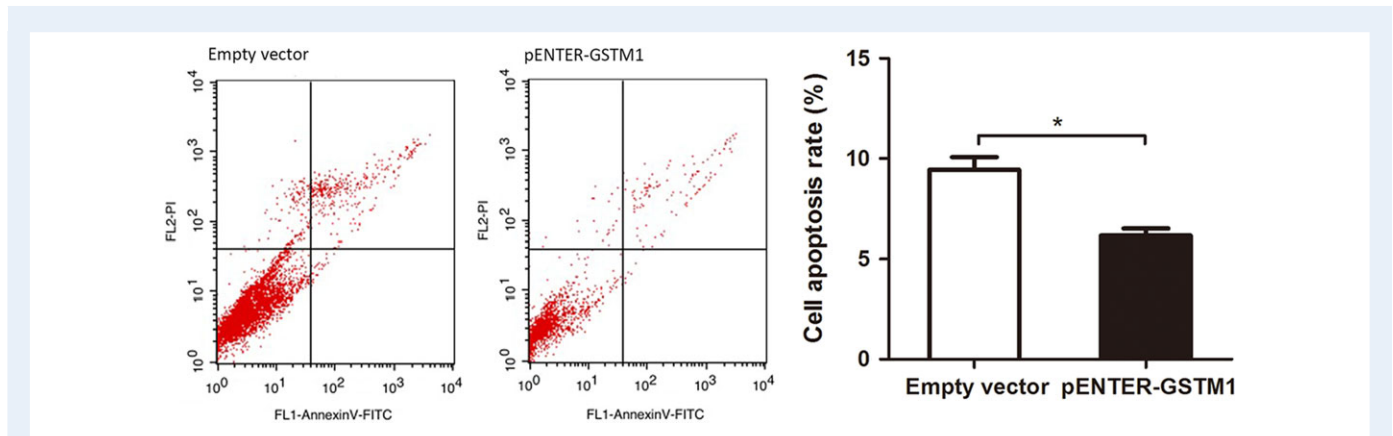
Figure 5 Effect of GSTM1 on endometrial epithelial cell (EEC) apoptosis following hormone treatment and withdrawal. Empty vector and pENTER- GSTM1 transfected EECs were treated with oestradiol and progesterone for 48 h; following the removal of hormones from the medium, cells were incubated for another 24 h. Thereafter, the flow cytometry analysis was performed to analyse cell apoptosis. All experiments were repeated three times. Values were expressed as mean \pm SEM, * P < 0.05.
