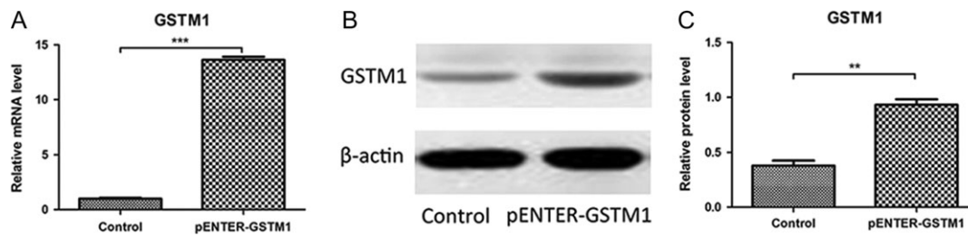
Figure 3 Effect of pENTER-GSTM1 on GSTM1 expression in endometrial epithelial cells (EECs). (A) Relative mRNA levels of GSTM1 in the pENTER-GSTM1 transfection group (pENTER-GSTM1 group) and empty vector transfection group (control group). (B) Protein expression of GSTM1 in the pENTER-GSTM1 transfection group (pENTER-GSTM1 group) and empty vector transfection group (control group). Data were expressed as mean \pm SEM, and analysed by Student's t test. All experiments were repeated three times. ** P < 0.01, *** P < 0.001.
