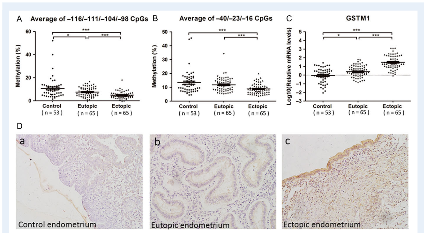
Figure 2 The expression and methylation analysis of GSTM1 in eutopic and ectopic endometrium of patients with ovarian endometriosis and the endometrium of women without endometriosis. (A, B) The average GSTM1 methylation levels of each fragment in the eutopic, ectopic and control endometrial tissues. * P < 0.05 , *** P < 0.001 . (C) Relative mRNA expression of GSTM1 in the eutopic, ectopic and control endometrial tissues. * P < 0.05 , *** P < 0.001 . (D) Representative immunohistochemical staining of GSTM1 in the endometrial tissues (SP \times 200). a: a case of endometrium from women without endometriosis demonstrating weak GSTM1 ; b: a case of eutopic endometrium from patients with ovarian endometriosis demonstrating moderate levels of GSTM1 ; c: a case of ectopic endometrium from patients with ovarian endometriosis demonstrating positive expression of GSTM1 .
